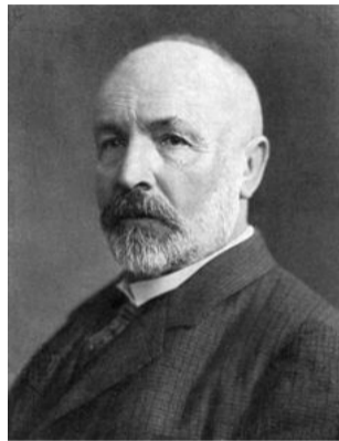
Georg Cantor (1845 – 1918) 1
