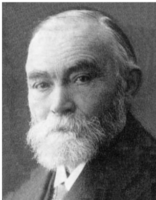
Gottlob Frege (1848 – 1925)
