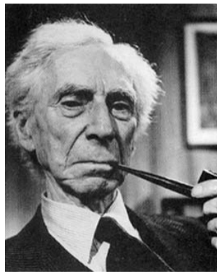
Bertrand Russell (1872 – 1970)
